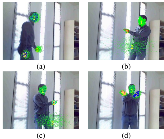
Fig. 2. Indicative tracking results in four frames of the office image sequence used in the previous example. In all cases the algorithm succeeds in correctly tracking the three skin-colored regions.
